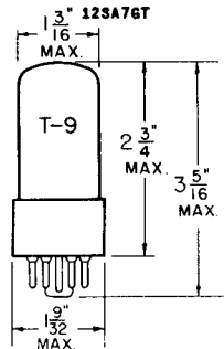
GLASS BULB
