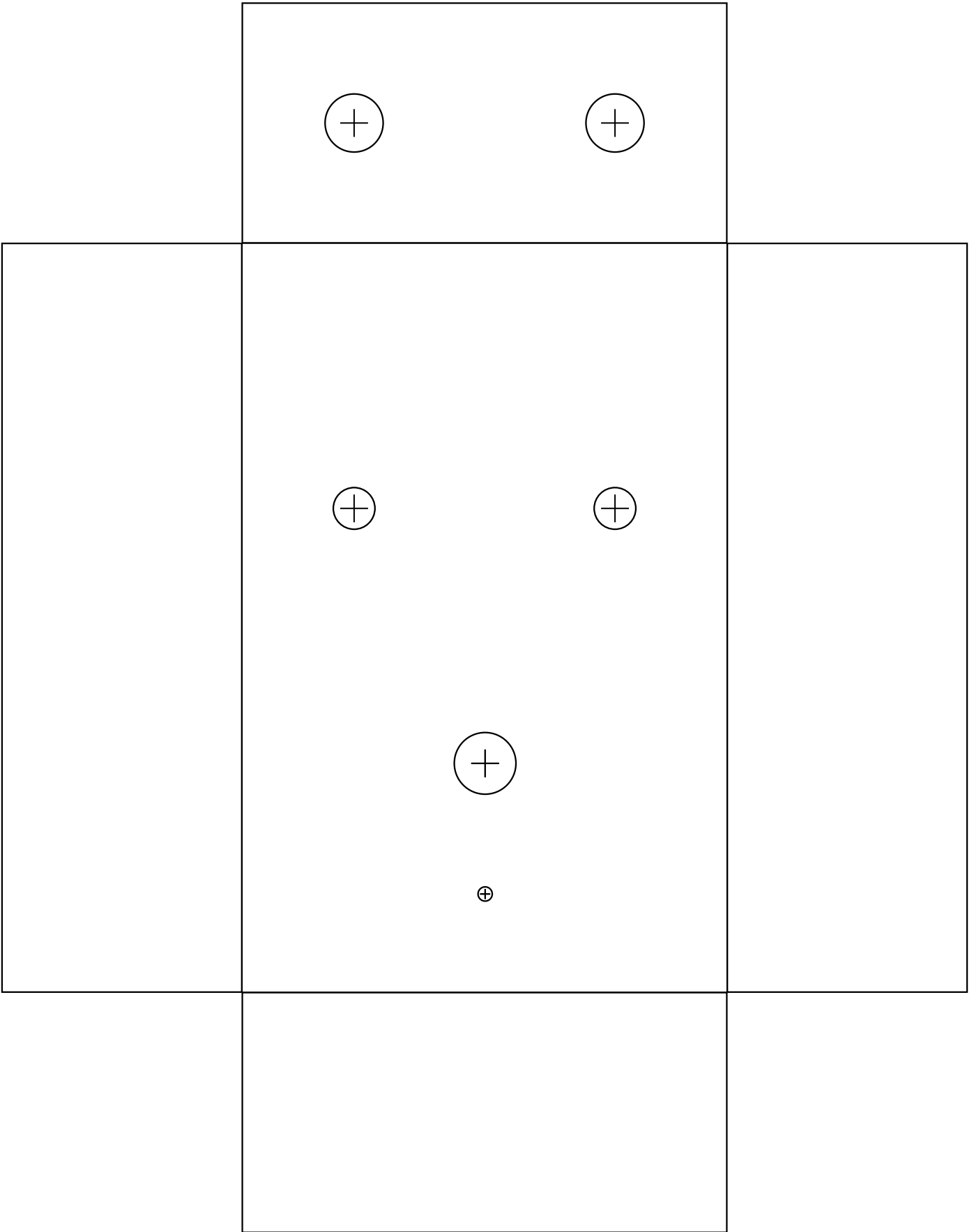
P-PKIT-BEND-MK2-X drill guide for the Hammond P-H1590J
