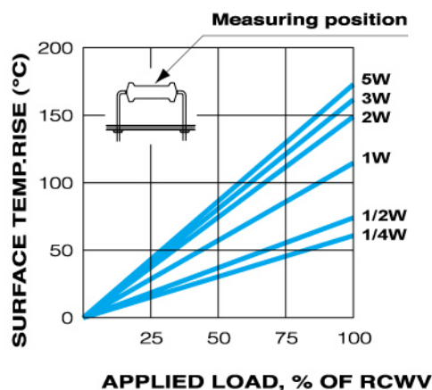
FIG.2 HOT-SPOT TEMPERATURE
