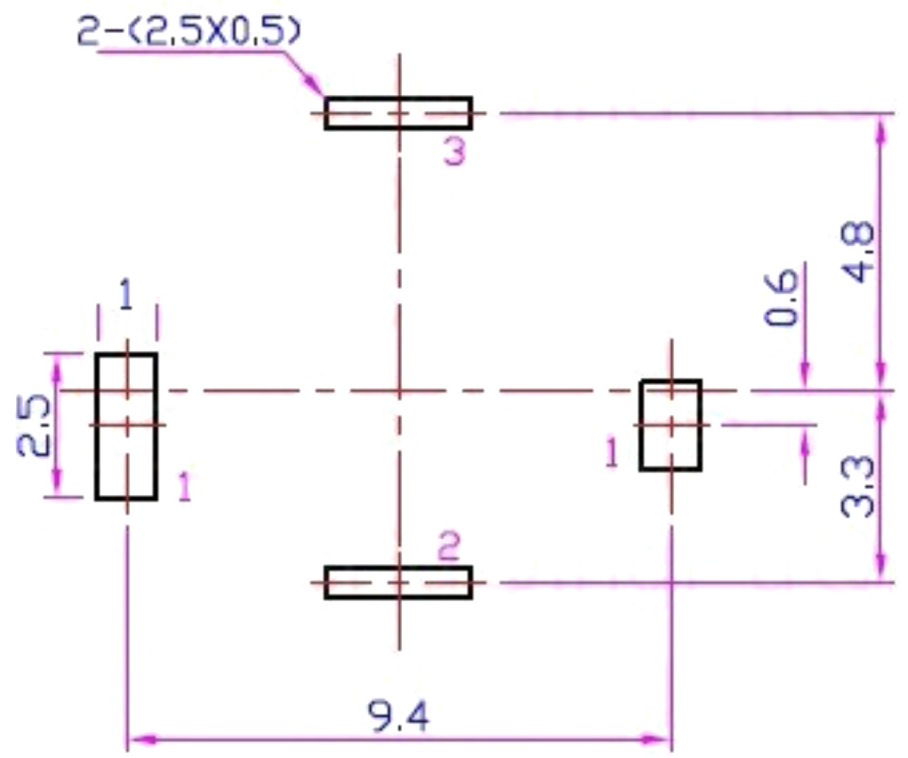
PCB LAYOUT (TOP VIEW)
